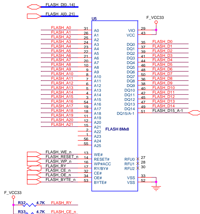
Figure 5.24. Flash schematic.
