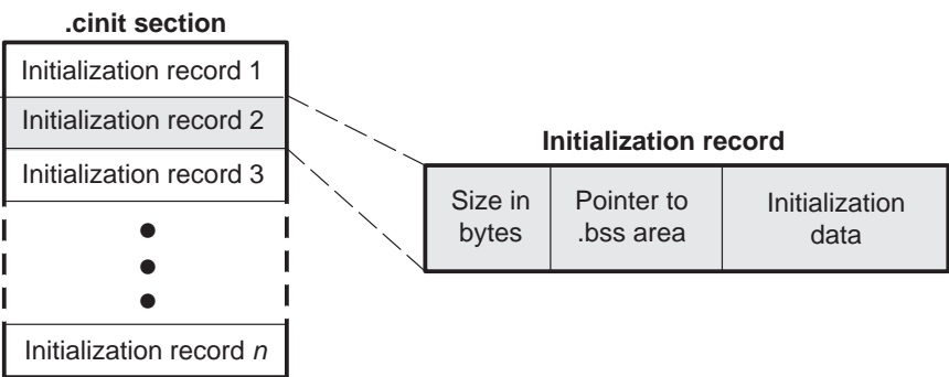
Figure 8–7. Format of Initialization Records in the .cinit Section
